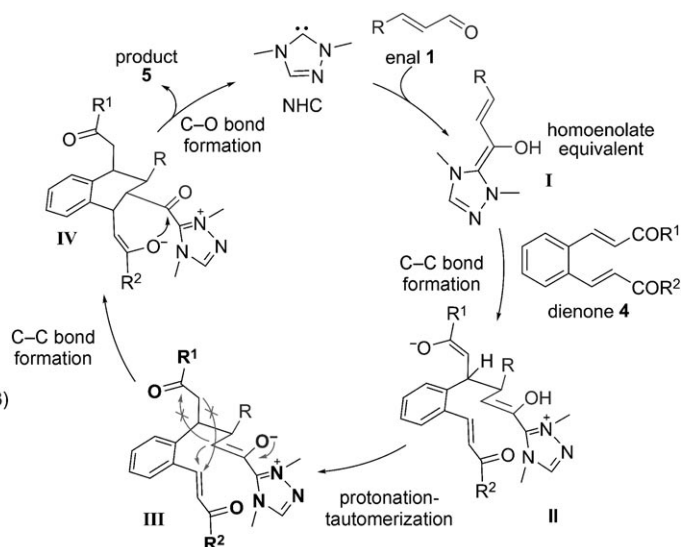
Scheme 1. Postulated catalytic pathways for NHC-mediated annulation of enals and di(enone)s.
